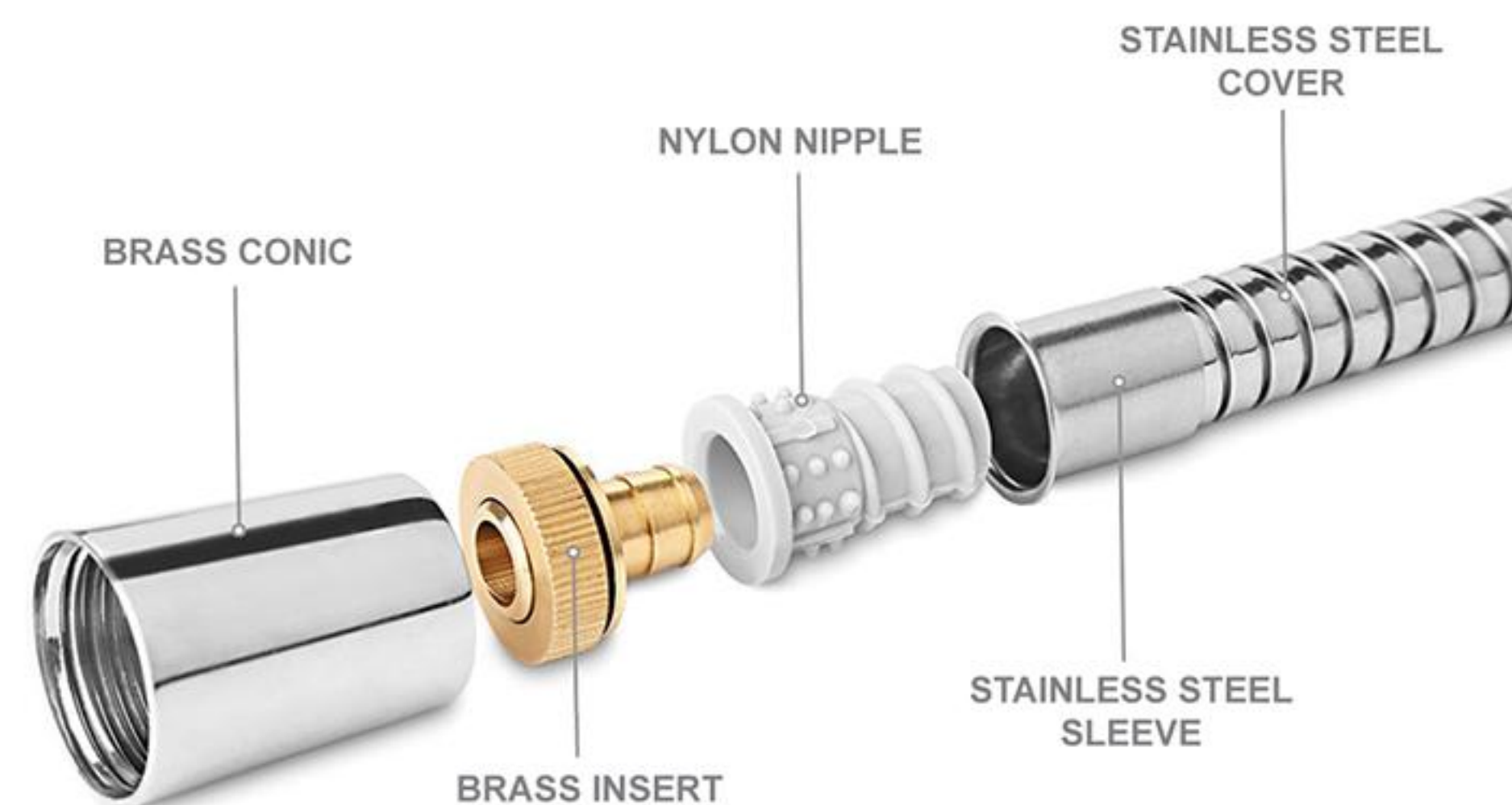
Interface Hose Length: 20 & 30 CM Dia: 12 MM / Size: 1/2" & 3/8" Material: SS - EPDM - Brass
